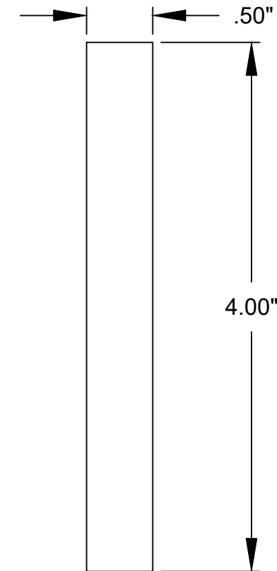
MULLION STIFFENER (6063-T5)
