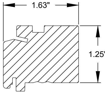
SASH STILE (PINE)
