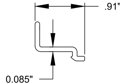
PICTURE CLIP (6063-T5) (VINYL)
