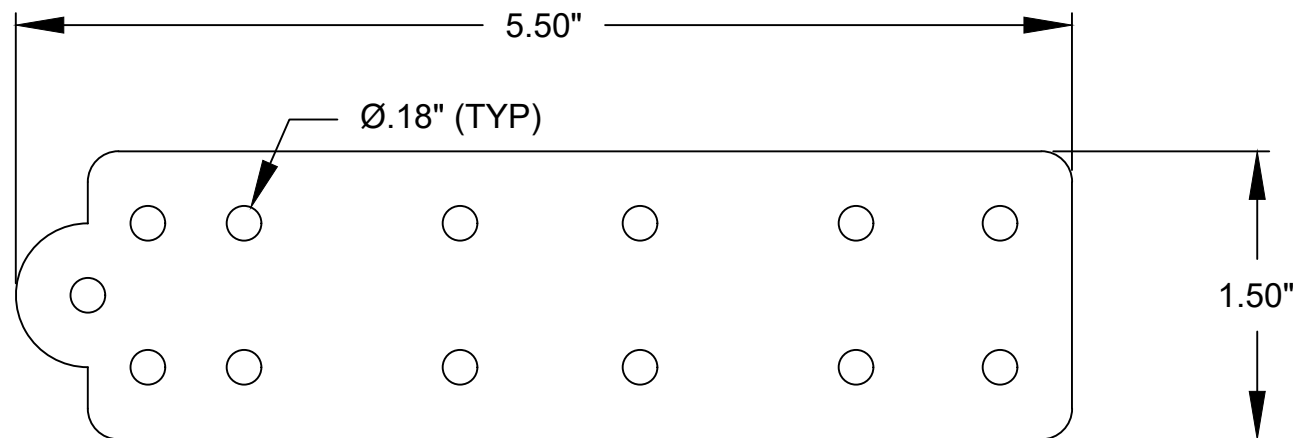
STRAP ANCHOR (20 GAGE STEEL)
