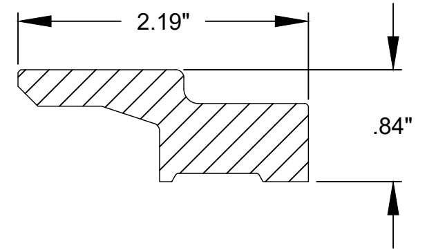
SIDE JAMB COVER (PINE)
