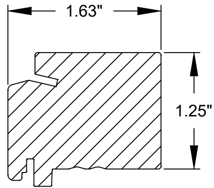
SASH RAIL (PINE)
