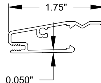
FRAME CLAD (6063-T5)
