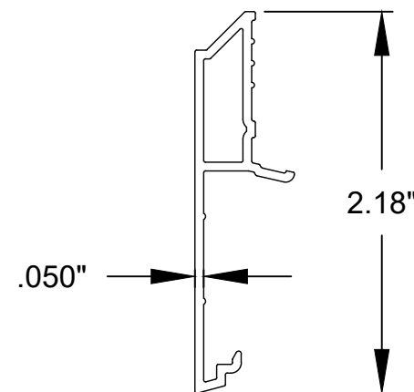
SASH CLAD (6063-T5)
