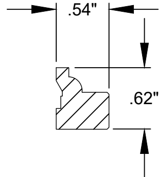
GLAZING BEAD (PINE)
